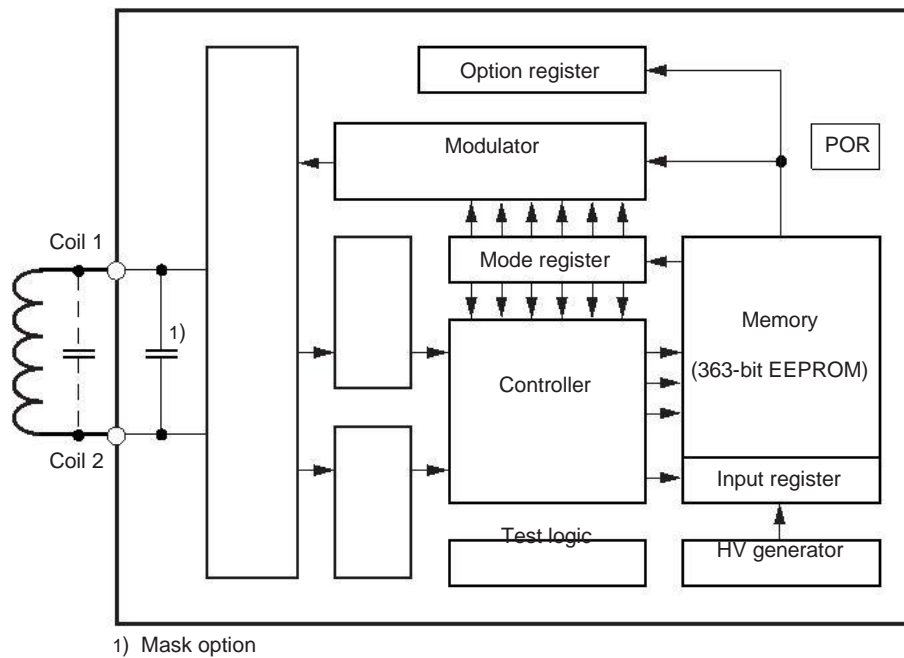
Figure 4-1. Block Diagram
